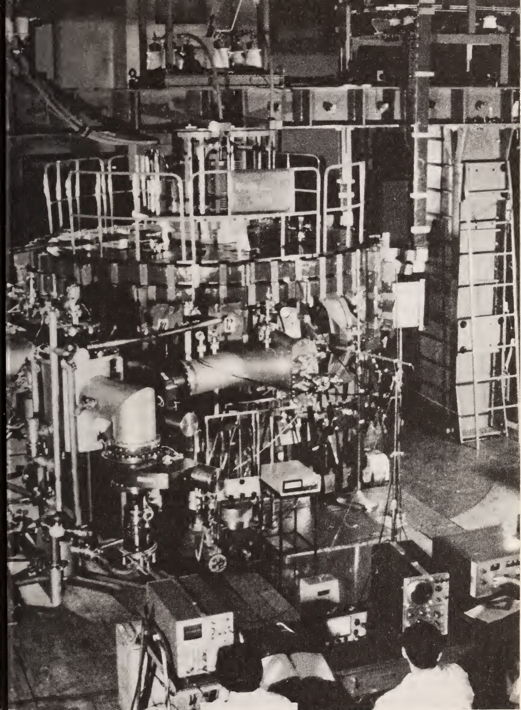
China's HL-1 controlled-nuclear fusion experimental device Courtesy Xinhua News Agency
